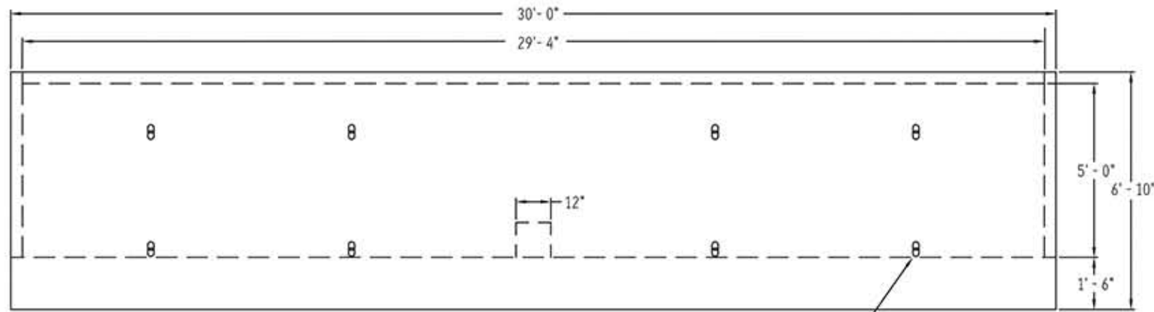
PLAN VIEW
